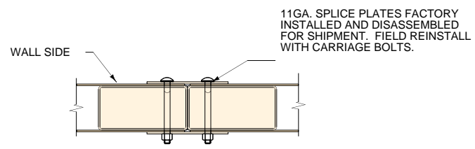
SPLICE PLATE DETAIL
