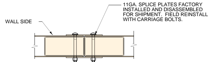
SPLICE PLATE DETAIL
