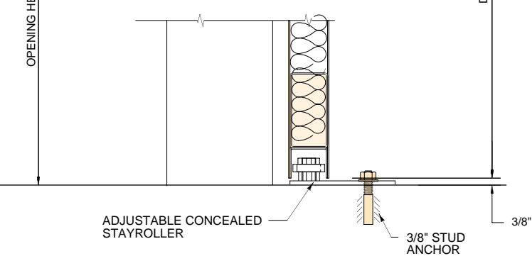
SILL DETAIL
