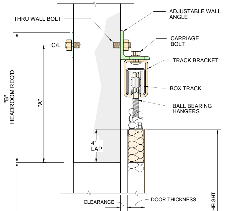
HEAD DETAIL
