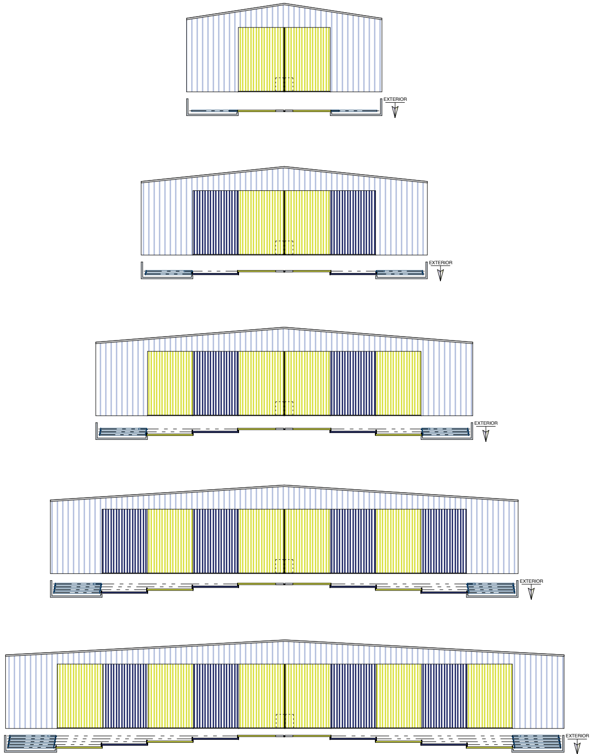
EXTERIOR ELEVATION & PLAN VIEWS @ THE H-SERIES MODEL HB200-HB1000 HANGAR DOORS
