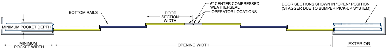
PLAN VIEW SHOWING DOOR SECTIONS NORTHERN STACK DESIGN SHOWN
