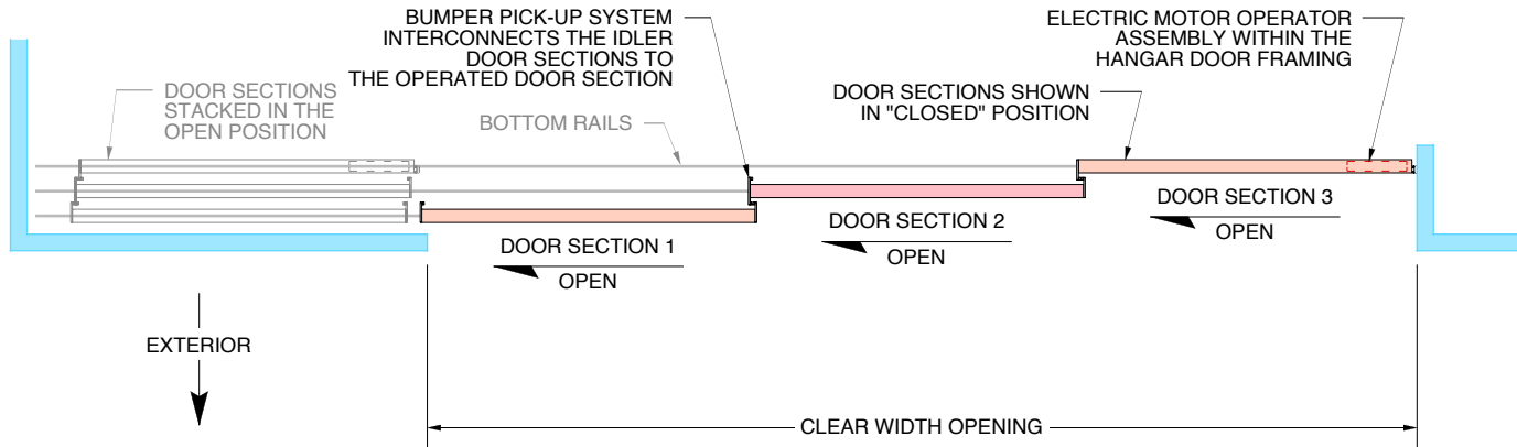
PLAN VIEW - H-SERIES, MODEL HU300
